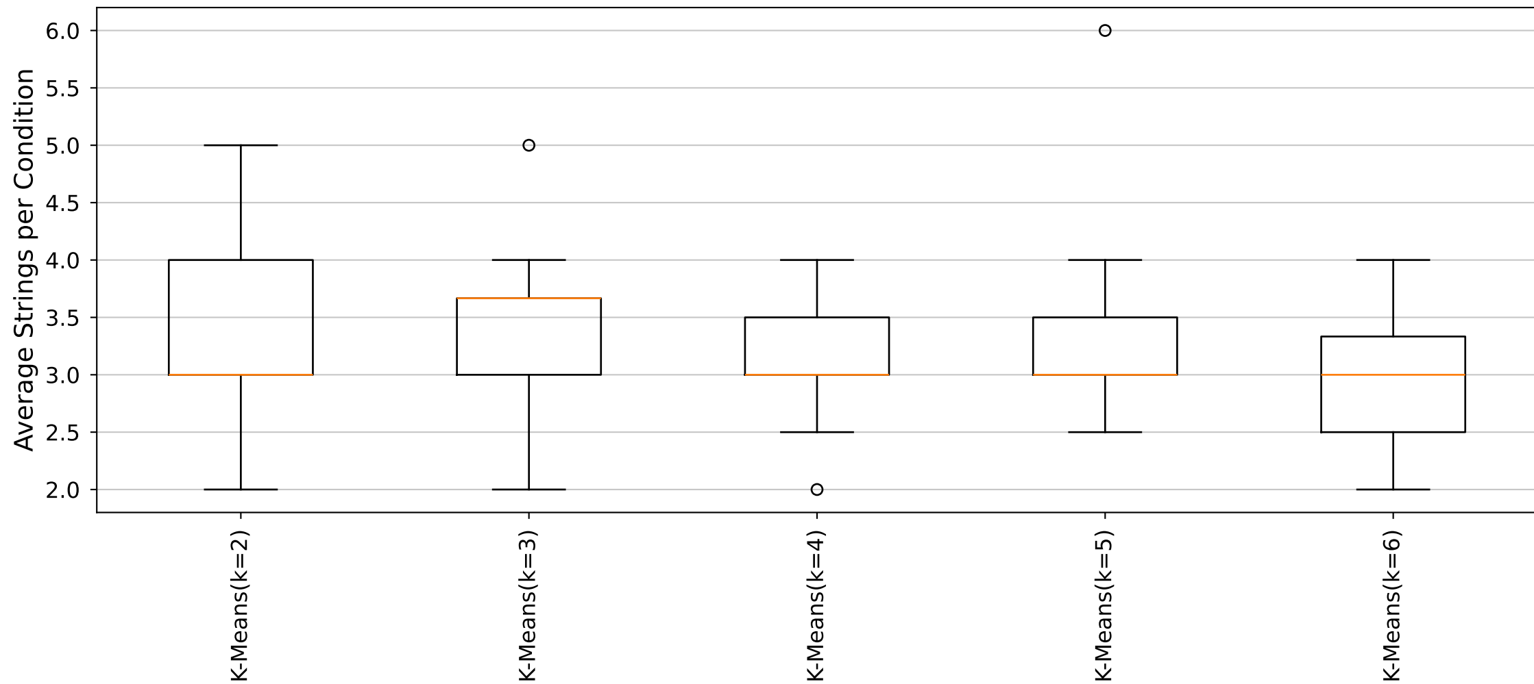
YARA Rules Average Strings per Condition Distribution (Cluster32_Size6 dataset)
